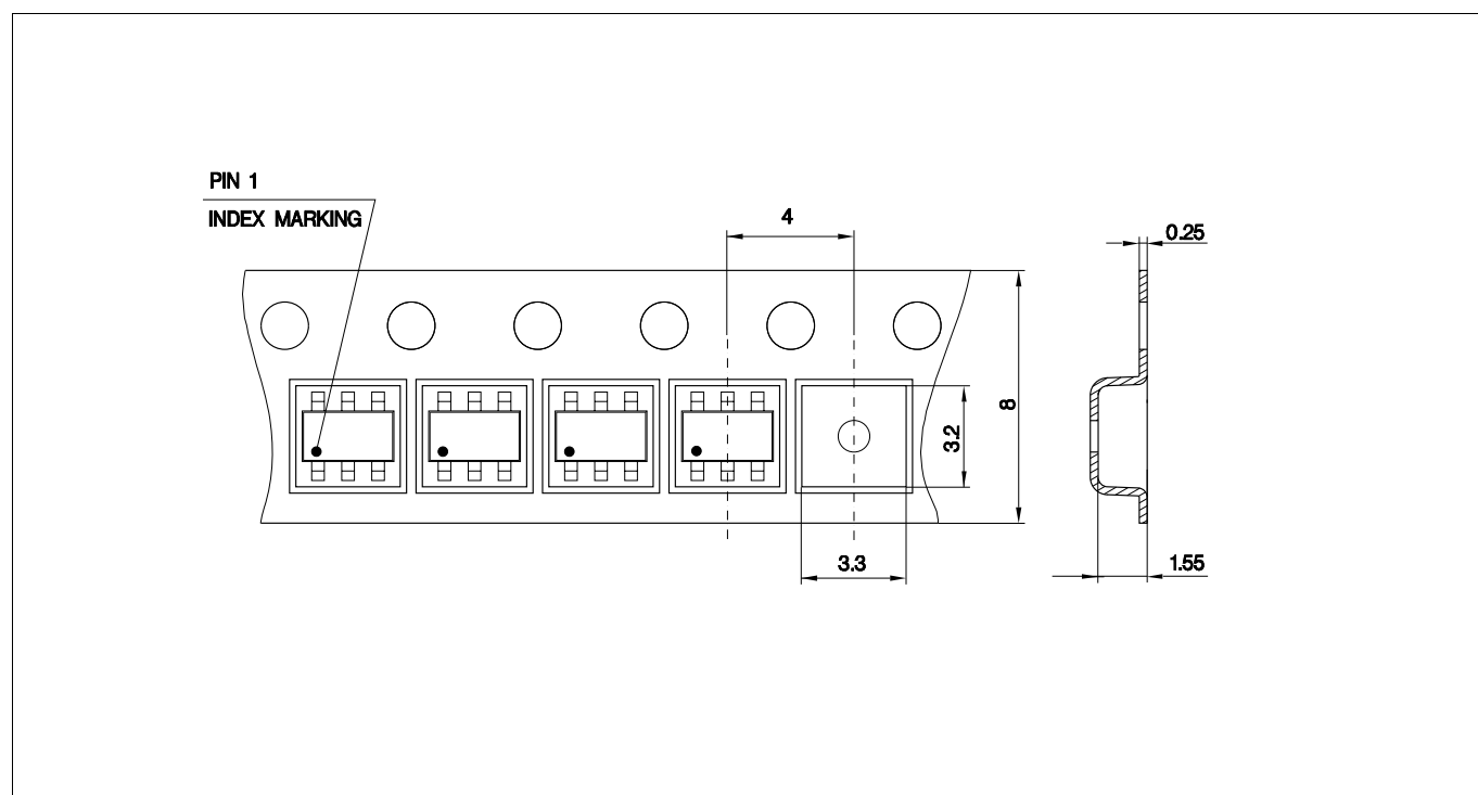
Figure 18 PG-SOT23-6-2 packaging dimensions
