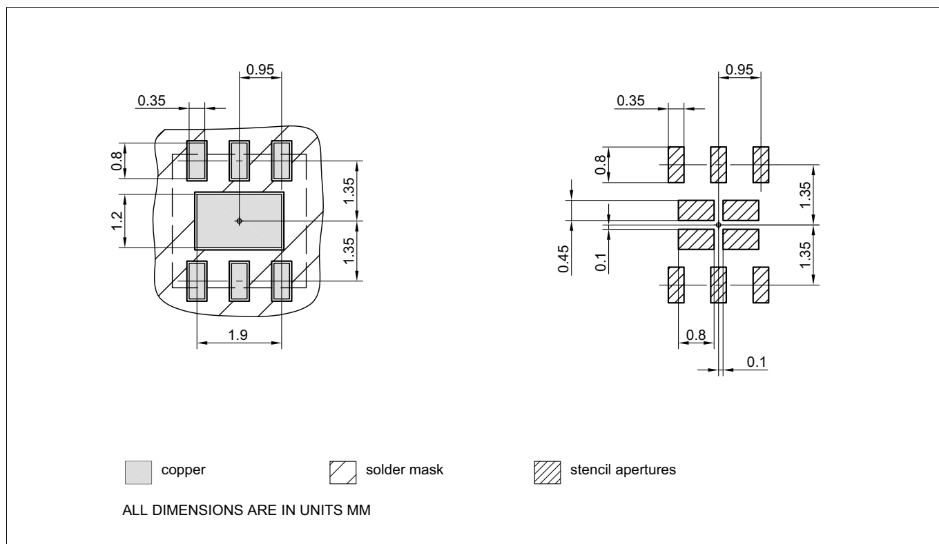
Figure 23 PG-WSO6-1 footprint dimensions
