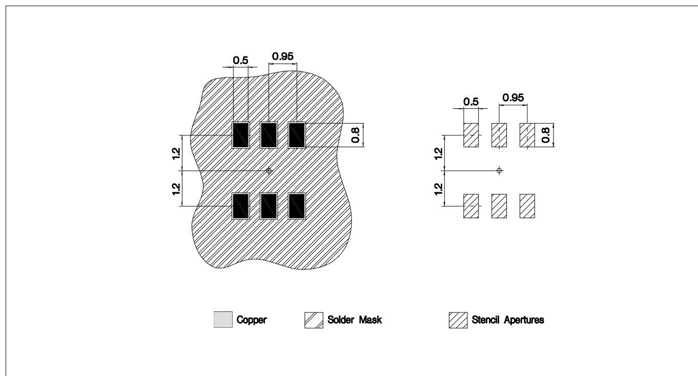
Figure 17 PG-SOT23-6-2 footprint dimensions
